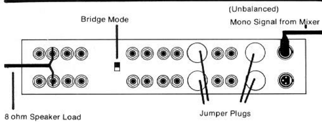
CS-1200 PATCH DIAGRAM 4 Bridge Mode Operation Unbalanced Low Z Input (Pin #3 Input)
